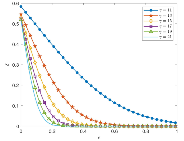
Figure 6 (Color online) Correlation between the proposed CRLB-based method and differential privacy.
