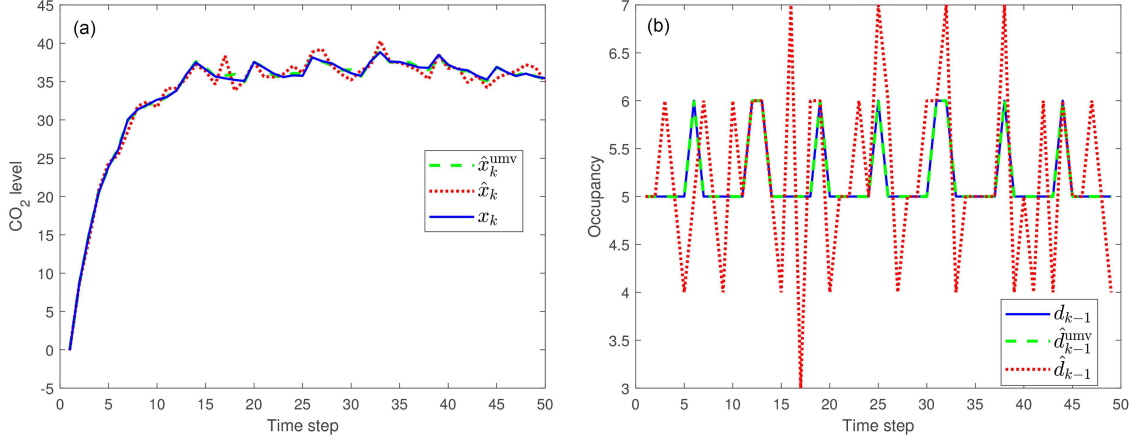
Figure 3 (Color online) CO 2 level, occupancy and their estimates. (a) CO 2 level and its estimates by an unbiased minimum-variance linear state estimator or privacy-preserving state estimator; (b) occupancy and its estimates by the adversary using an unbiased minimum-variance linear state estimator or privacy-preserving state estimator.
