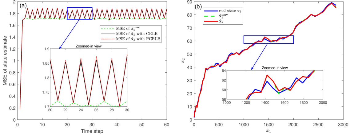
Figure 4 (Color online) Comparison of unbiased minimum-variance linear state estimates and privacy-preserving state estimates. (a) MSEs of unbiased minimum-variance linear state estimates and privacy-preserving state estimates; (b) trajectories of real states, unbiased minimum-variance linear state estimates, and privacy-preserving state estimates.
