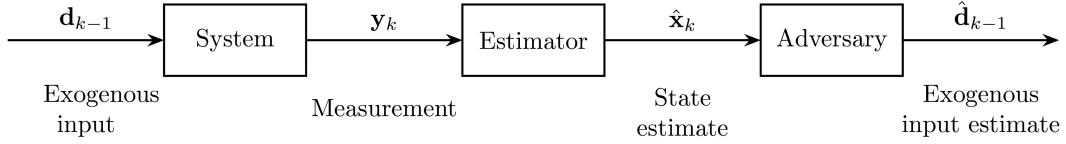
Figure 1 The privacy-preserving state estimation setup.
