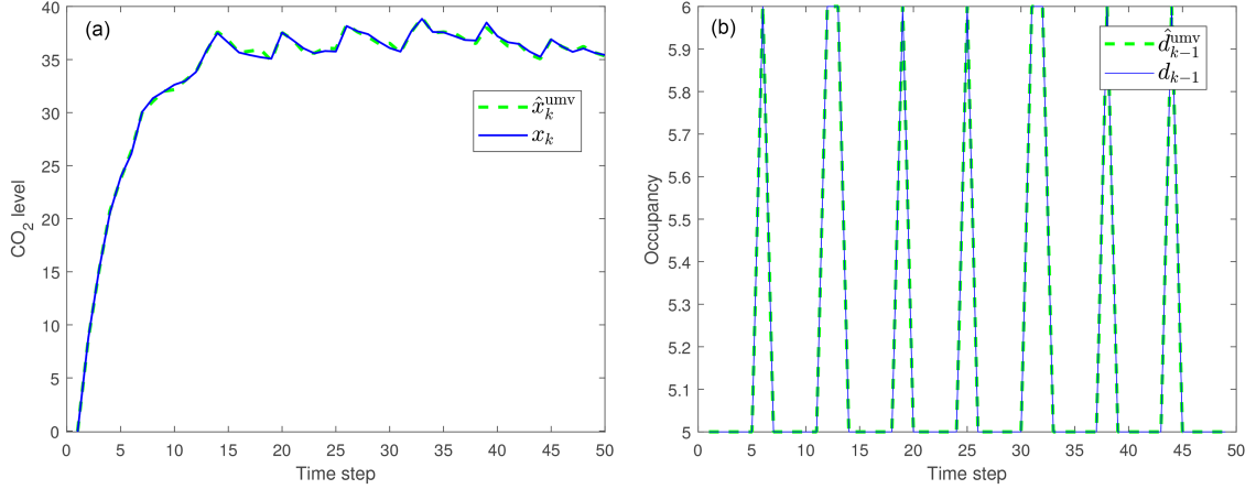
Figure 2 (Color online) CO 2 level, occupancy and their estimates. (a) CO 2 level and its estimate by the unbiased minimum-variance linear state estimate; (b) occupancy and its estimate by the adversary using (6).
