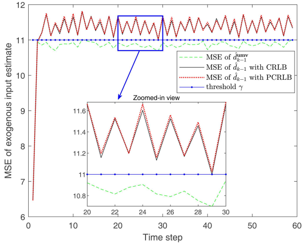
Figure 5 (Color online) MSEs of the adversary's estimates for d_k with either an unbiased minimum-variance linear state estimator or a privacy-preserving state estimator.
