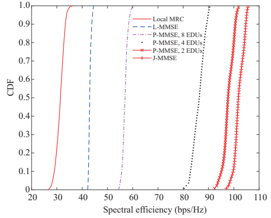
Figure 9 (Color online) CDF of the total spectral efficiency of the system with 12 data streams.
