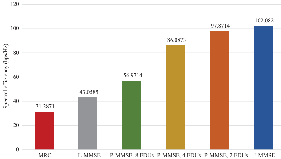
Figure 10 (Color online) Average total spectral efficiency of the system with 12 data streams.
