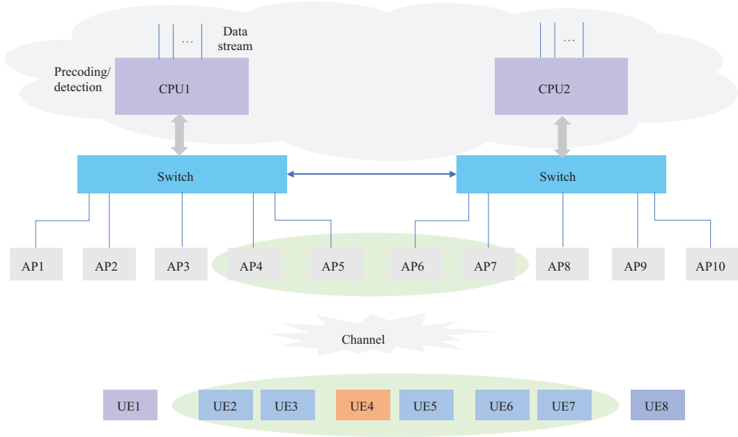
Figure 1 (Color online) DCC-based CF-mMIMO implementation architecture.
