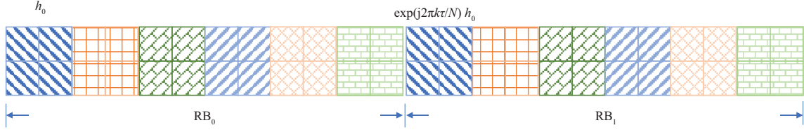
Figure 5 (Color online) A pattern of a 24-port orthogonal DMRS.
