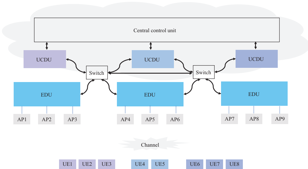
Figure 3 (Color online) A novel CF-mMIMO architecture.
