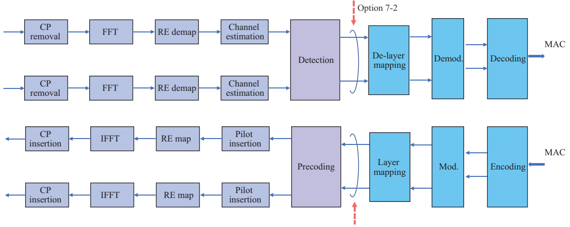
Figure 4 (Color online) Physical-layer signal processing and splitting Option 7-2 of 5G new radio (NR).
