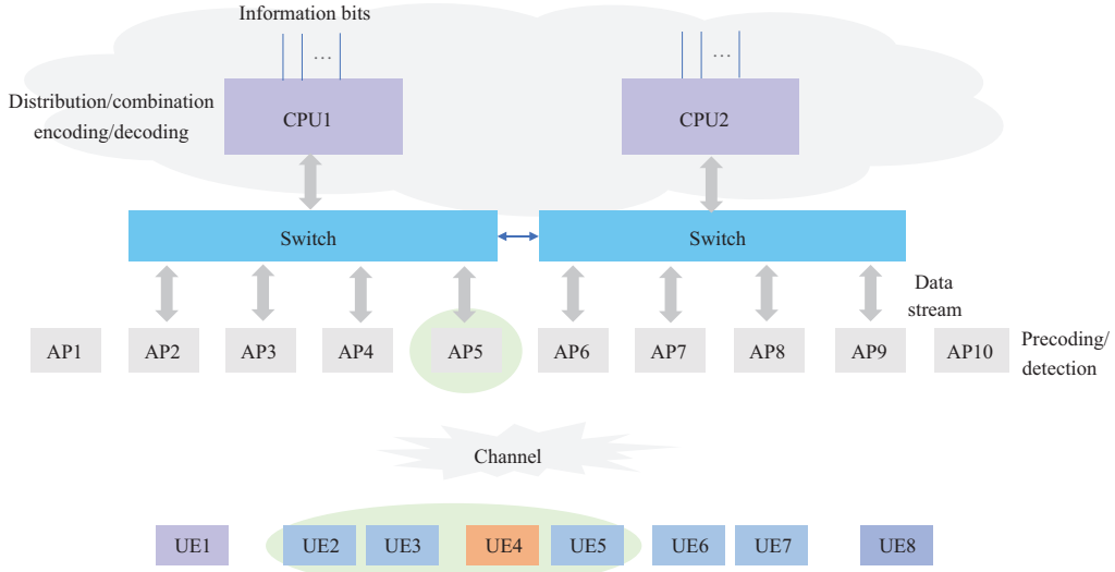
Figure 2 (Color online) Fully distributed CF-mMIMO implementation architecture.
