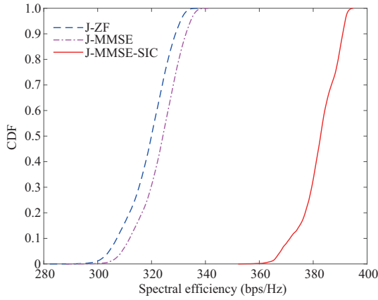
Figure 8 (Color online) Total spectral efficiency of the system with 48 data streams.
