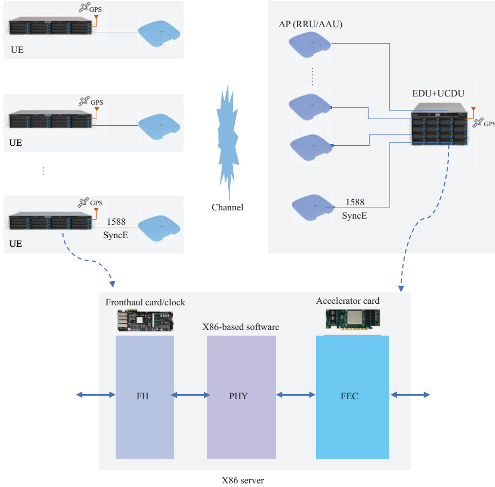
Figure 6 (Color online) Schematic diagram of the prototype full-spectrum CF-RAN system.
