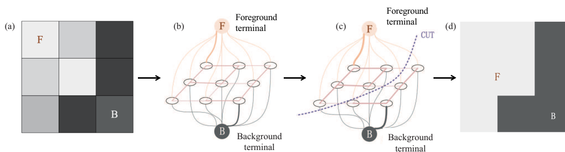
Figure 2 (Color online) (a) A simple 3×3 image with two seed pixels. The pixel marked with “F” represents “foreground” seed while the other one represents “background” seed, and the remaining pixels are unknown. (b) The constructed graph in which the cost of each edge is reflected by the edge’s thickness. (c) The min-cut algorithm tends to cut the edges with minimum costs. (d) Segmentation results.
