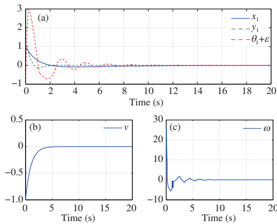
Figure 1 (Color online) (a) Trajectories of the system states; (b) control input u_0 ; (c) control input u .
