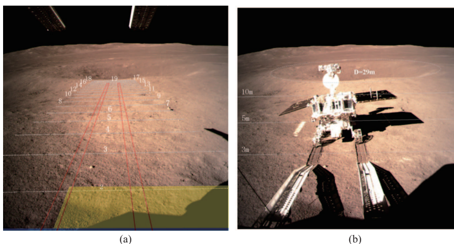
Figure 12 (Color online) Monoscopic measurement supporting the separation of the rover from the lander (the measurement and analysis results of rover landed before (a) and after (b)).
