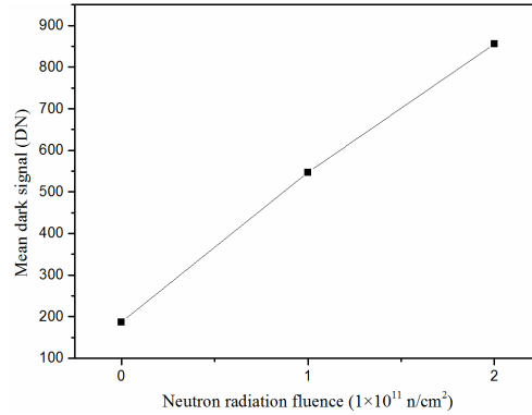
Fig. 5 The mean dark signals of the PPD CMOS image sensor reactor versus neutron radiation fluence.
