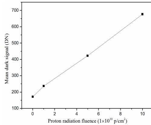
Fig. 7 The mean dark signals of the PPD CMOS image sensor versus proton radiation fluence.
