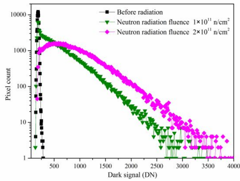
Fig. 4 The dark signal distributions induced by neutron radiation.
