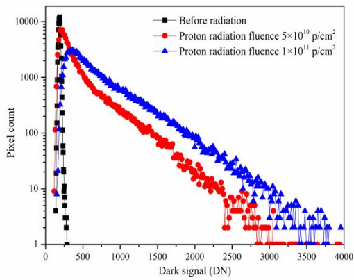
Fig. 6 The dark signal distributions induced by proton radiation.
