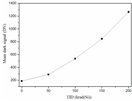
Fig. 1 The mean dark signals of the PPD CMOS image sensor versus the TID.
