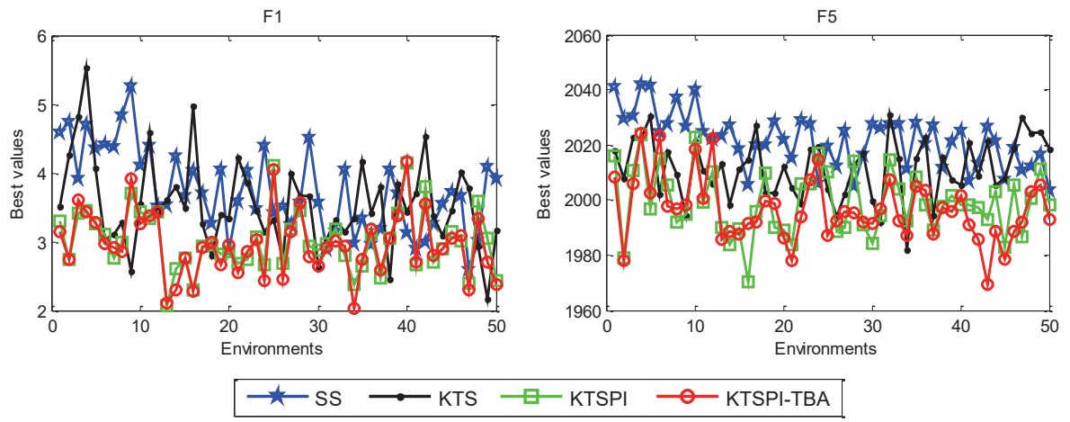
Figure A2 The average result over 20 independent runs of each environment on F1 and F5.
