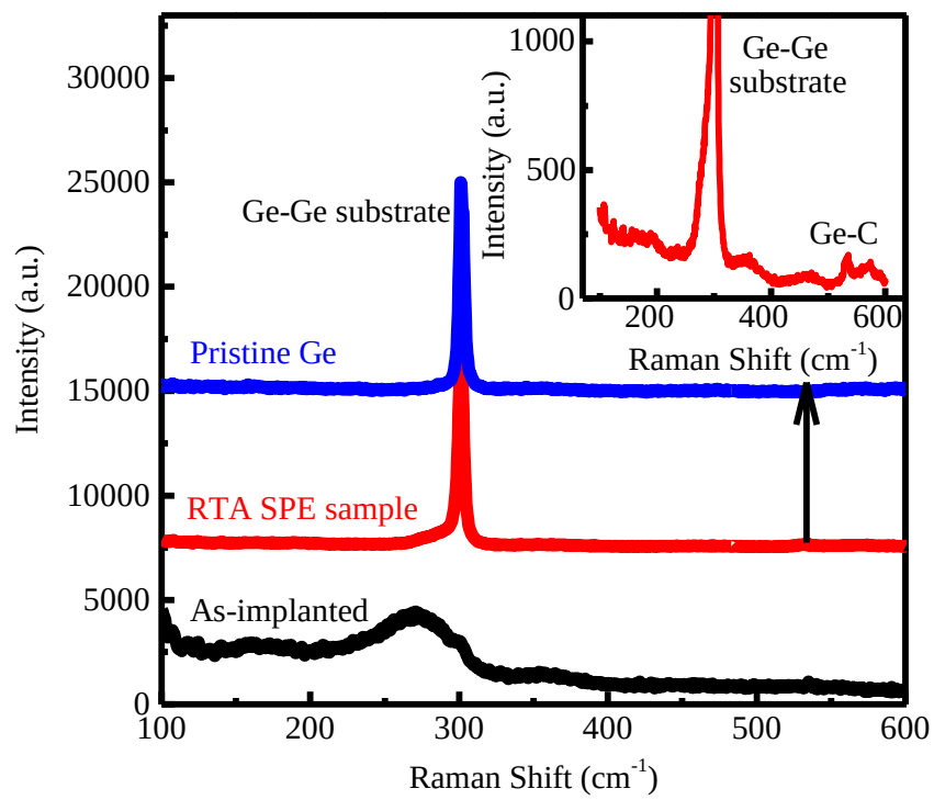
Raman spectrum of as-implanted SPE sample, RTA sample (500 ^{\circ}\text{C} , 600 s) and pristine Ge
