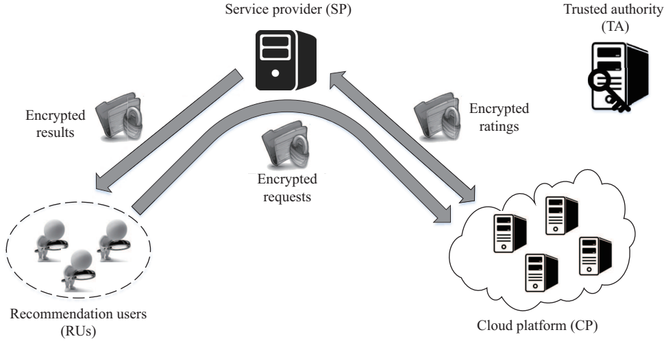
Figure 1 System Framework of APPLET.
