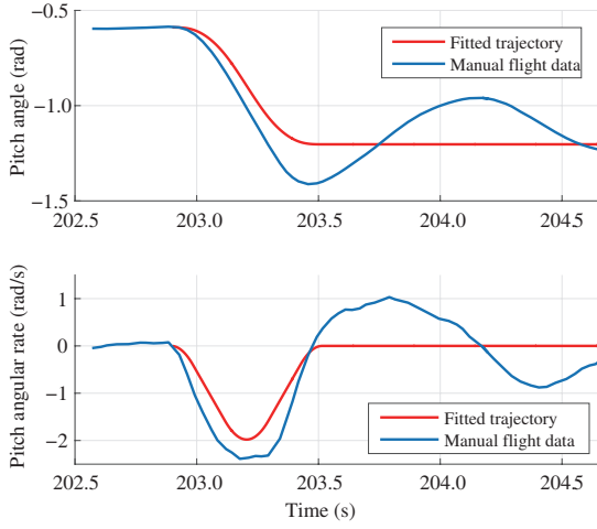
Figure 9 (Color online) Manual forward transition data.
