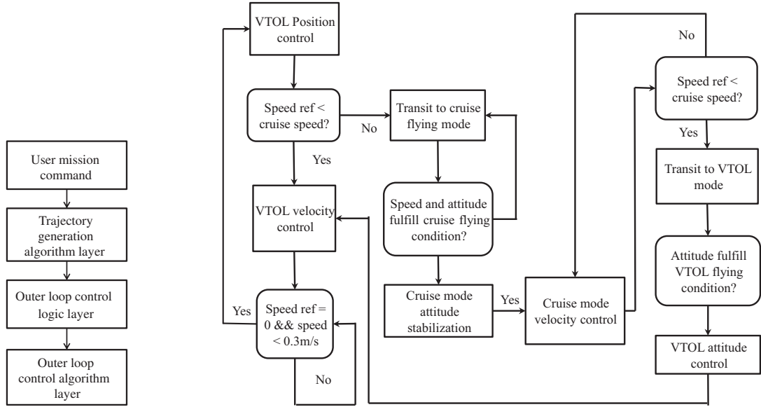
Figure 11 Outer loop overall structure.
