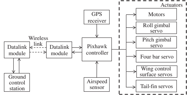
Figure 3 Avionics system.
