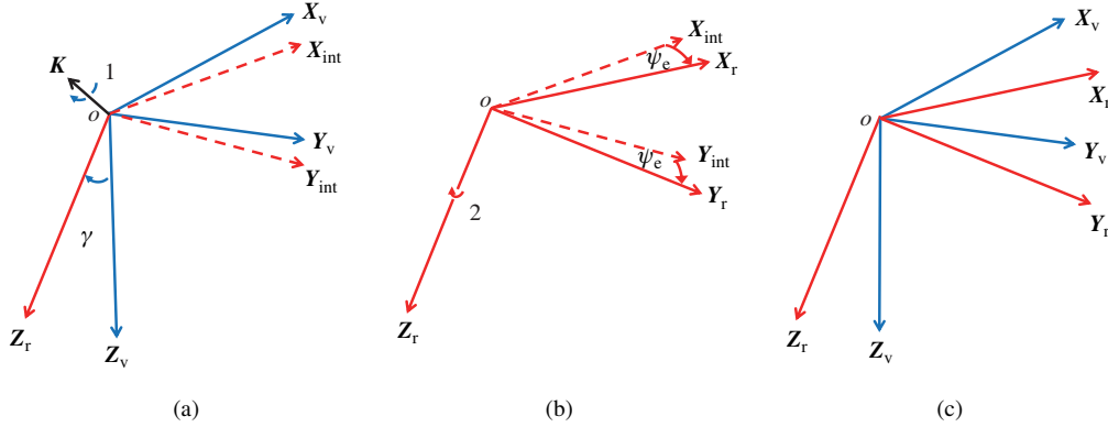
Figure 6 (Color online) The body frame rotation angle generating logic. (a) Align Z_v -axis with the Z_r -axis by rotating about the K -axis which is perpendicular to the two axes by an angle of \gamma and results in an intermediate frame F_{int} ; (b) rotate the frame F_{int} about Z_r -axis by an angle of \psi_e to reach the reference axis; (c) the original frame F_v and the reference frame F_r .
