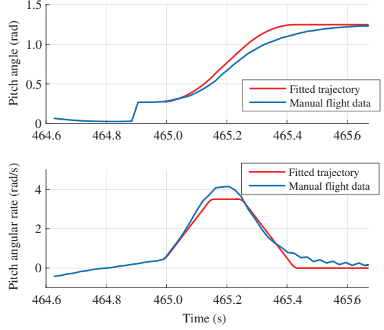
Figure 10 (Color online) Manual backward transition data.
