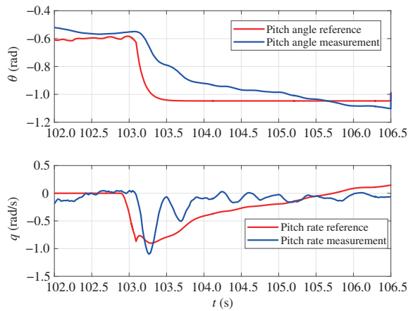
Figure 17 (Color online) Forward transition pitch angle data.
