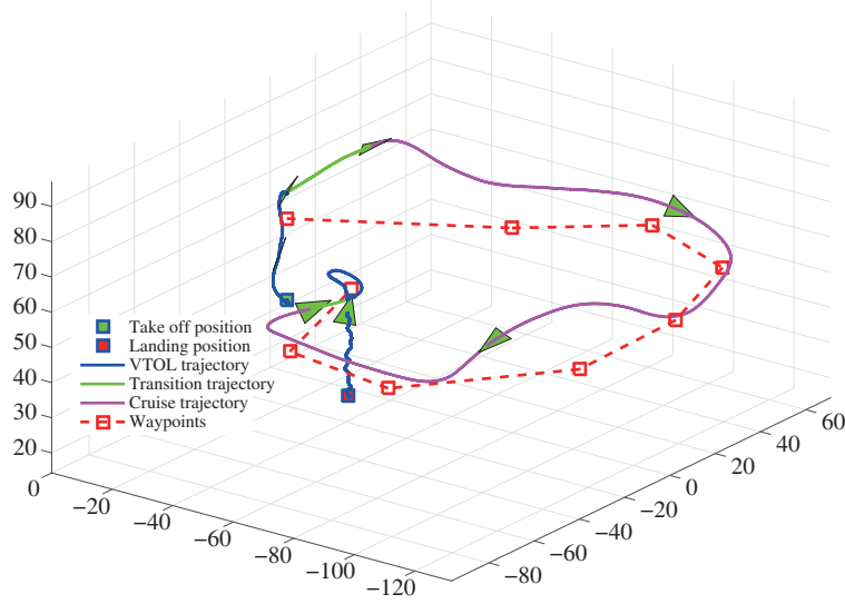
Figure 14 (Color online) The position result for the fly test.
