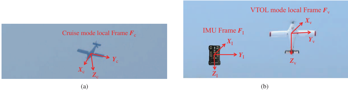
Figure 4 (Color online) The two local frames proposed. (a) U-Lion cruise flying frame; (b) U-Lion VTOL flying frame.
