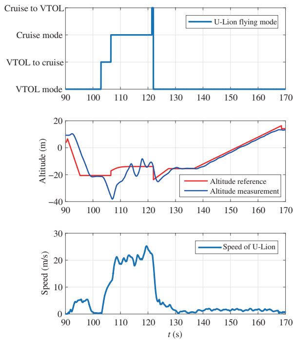
Figure 15 (Color online) Flight data.
