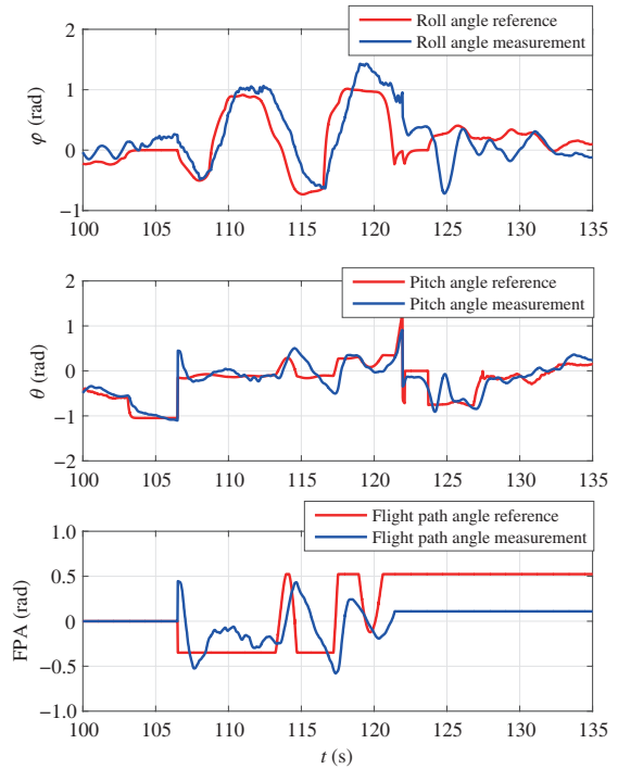
Figure 16 (Color online) Flight angle data.
