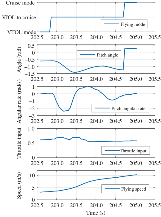
Figure 7 (Color online) Manual forward transition data.
