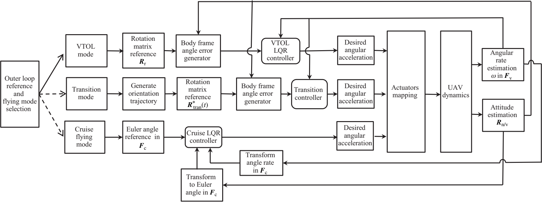
Figure 5 The inner loop control structure.
