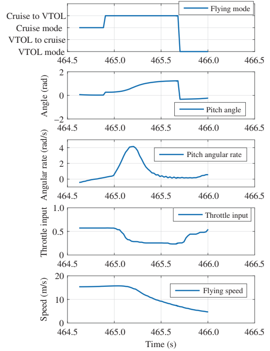
Figure 8 (Color online) Manual backward transition data.
