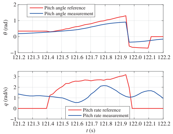
Figure 18 (Color online) Backward transition pitch angle data.
