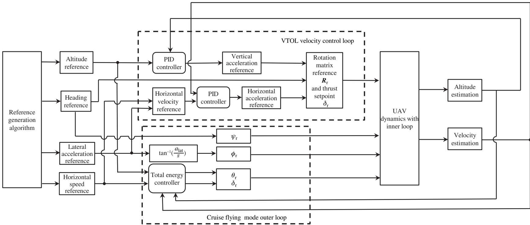
Figure 13 The outer loop control structure.
