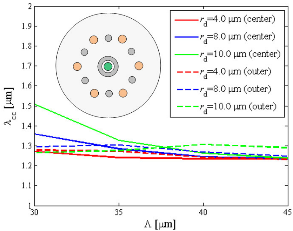
Figure S1 Dependence of \lambda_{cc} on \Lambda and r_o for 7-trench assisted 7-core fiber
