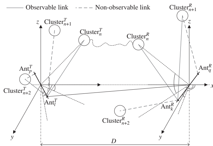
Figure 2 A 3-D wideband twin-cluster massive MIMO channel model in [54].
