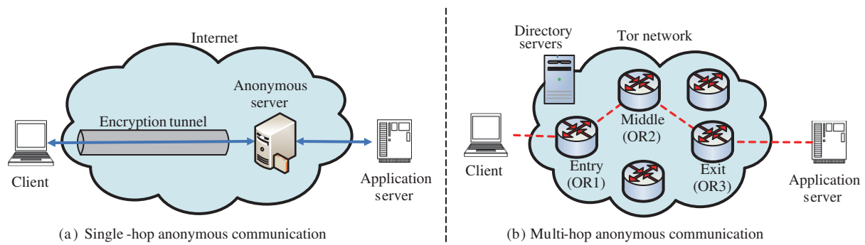
图 3 (网络版彩图) 匿名通信系统架构 Figure 3 (Color online) Anonymous communication models
